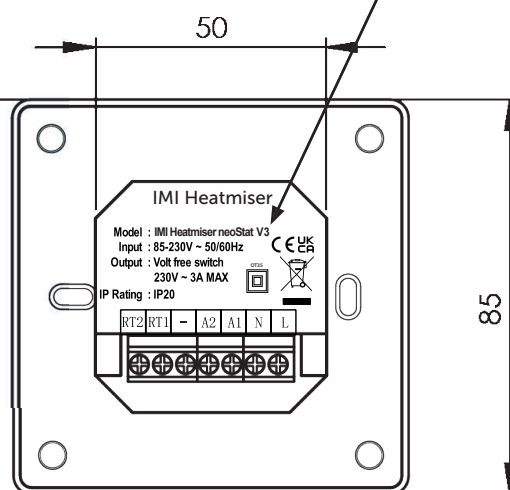
Wiring Detail
