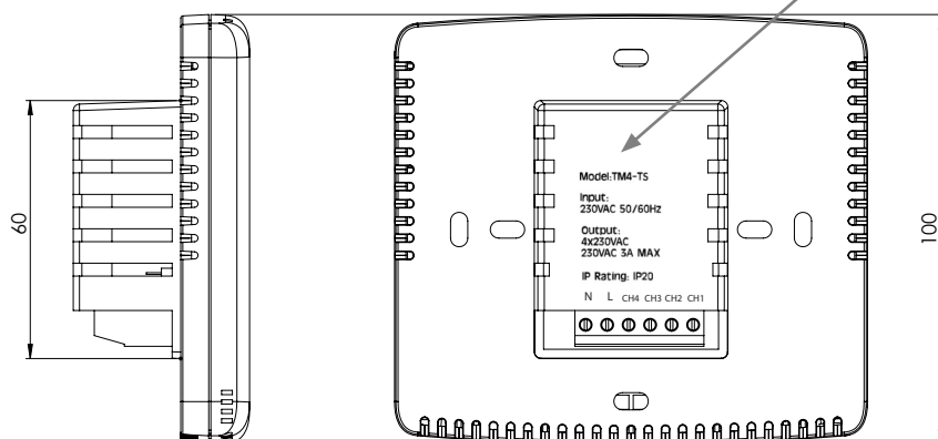
Bedrading detail
