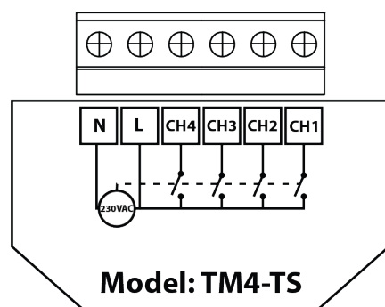
Bedrading detail
