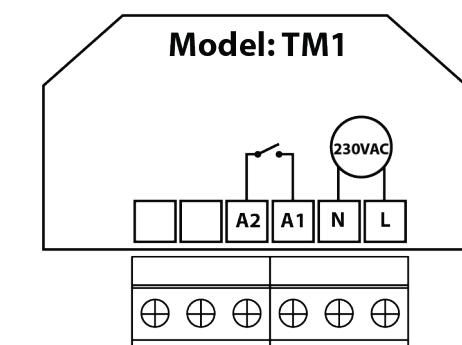
Bedrading detail
