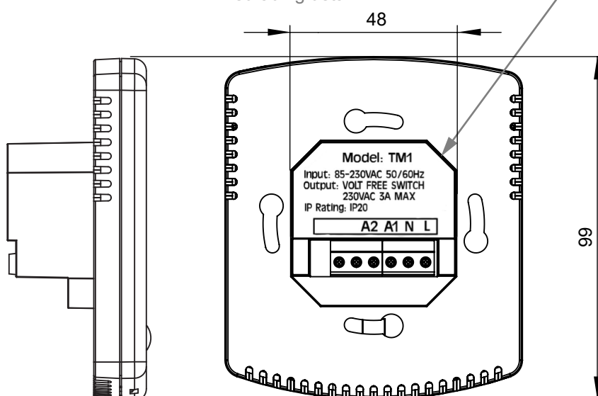
Bedrading detail
