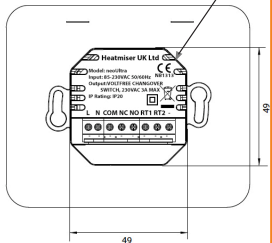
Bedrading detail
