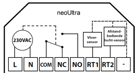
Bedrading detail
