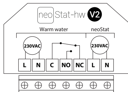
Bedrading detail
