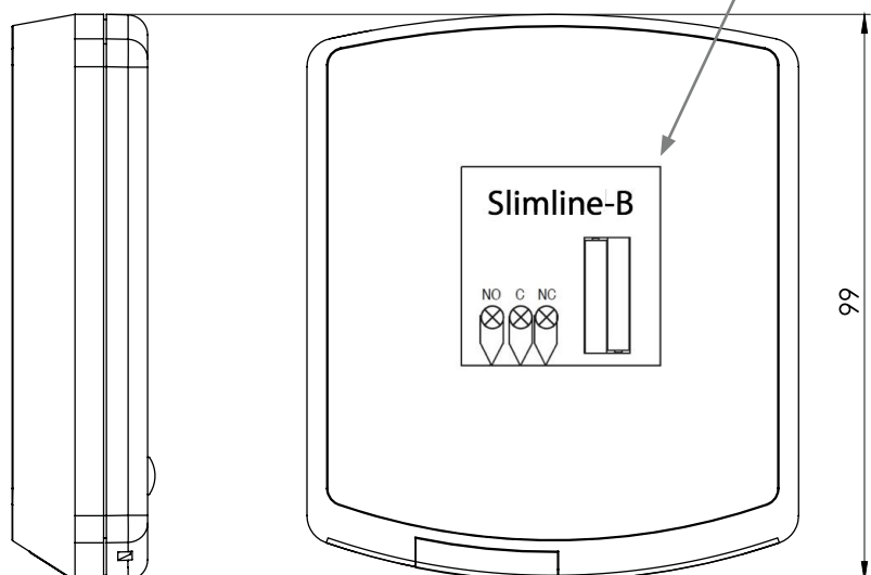
Bedrading detail
