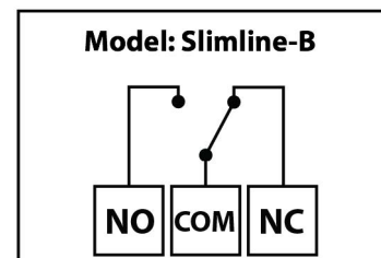
Bedrading detail
