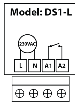
Bedrading detail
