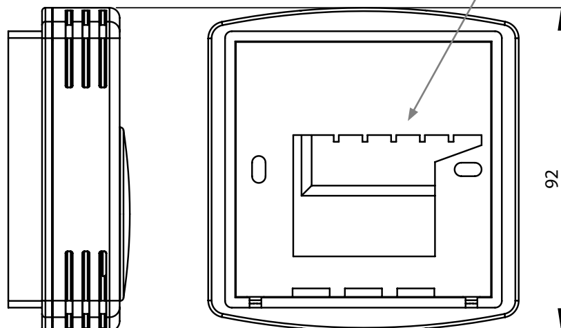
Bedrading detail
